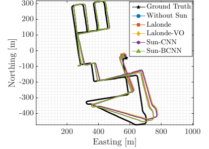
(c) 08: VO and ground truth trajectories
