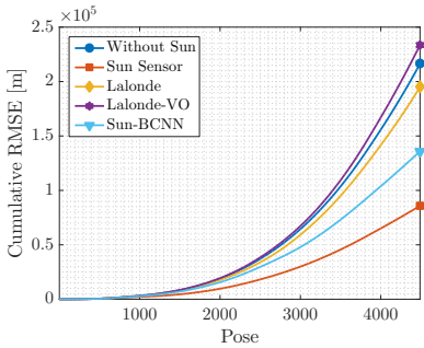
(g) 00: Translational CRMSE (EN-Plane)
