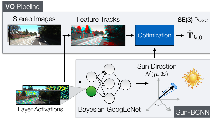
Figure 3.1: Our method uses a Bayesian Convolutional Neural Network (BCNN) to estimate the direction of the sun and to produce a principled uncertainty estimate for each prediction. We incorporate this ‘virtual sun sensor’ into a stereo visual odometry pipeline to reduce estimation error.
