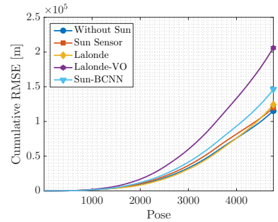
(i) 05: Translational CRMSE (EN-Plane)
