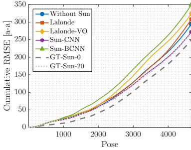
(g) 02: Rotational CRMSE
