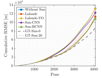
(f) 08: Translational CRMSE (EN-plane)
