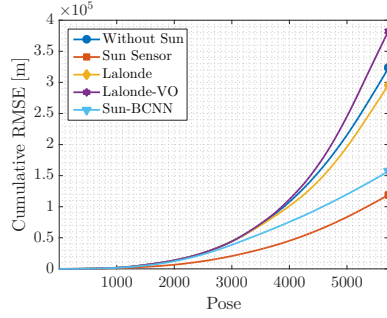
(e) 01: Translational CRMSE
