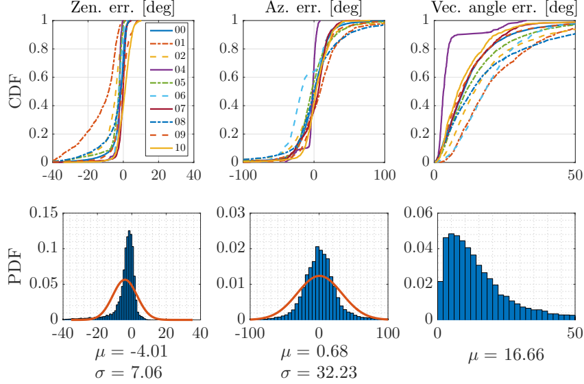
Figure 3.9: Distributions of zenith error, azimuth error, and angular distance for Sun-BCNN compared to ground truth for each test sequence in the KITTI dataset. Top row: Cumulative distributions of errors for each sequence individually. Bottom row: Histograms and Gaussian fits of aggregated errors.
