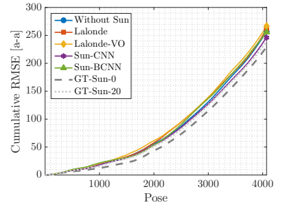
(i) 08: Rotational CRMSE
