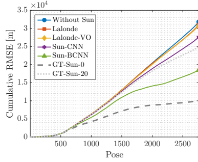
(e) 05: Translational CRMSE (EN-plane)
