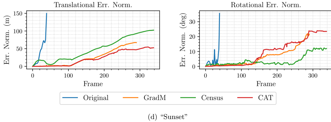
Figure 4.9: Comparison of metric localization errors on the VKITTI/0018 trajectory (continued from previous page).
