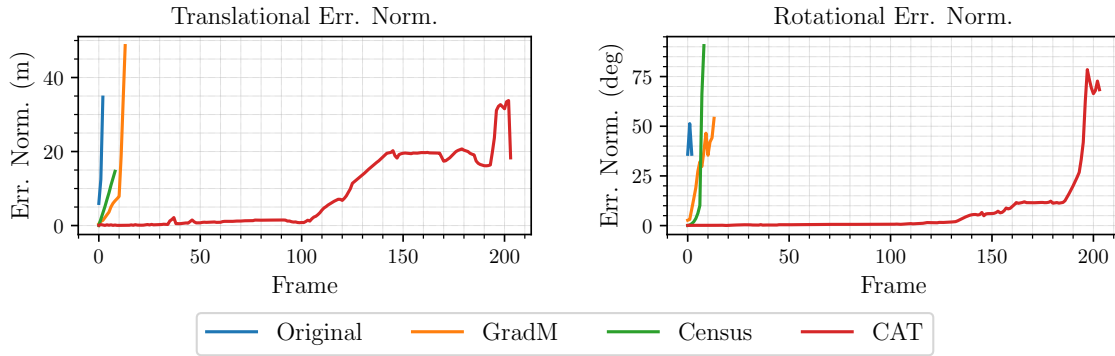
Figure 4.9: Comparison of metric localization errors on the VKITTI/0018 trajectory (continued on next page).
