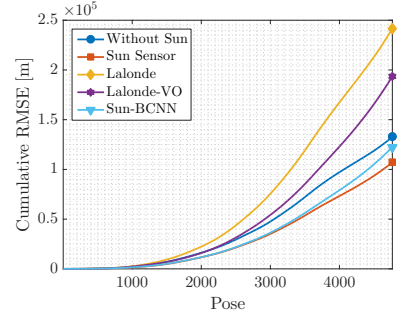
(f) 05: Translational CRMSE
