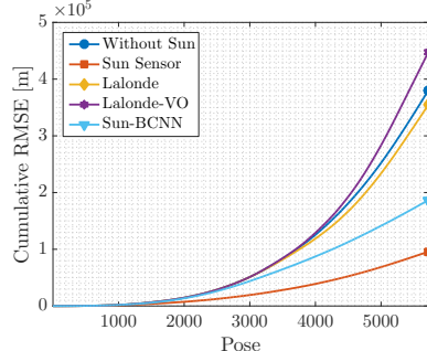
(h) 01: Translational CRMSE (EN-Plane)
