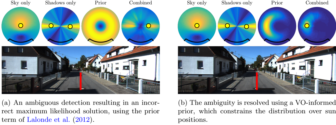
Figure 3.2: Sample frame from KITTI sequence 2011_09_30_drive_0018 and associated sun detection results using the “Lalonde” (Lalonde et al., 2012) and “Lalonde-VO” methods. Top row : Probability distributions over sun positions are shown for each visual cue independently, and for the combined result, with blue representing regions of low probability and yellow representing regions of high probability. The maximum likelihood solution(s) are represented as yellow circles, and the camera’s field of view is shown in black. Bottom row : A virtual sundial (red line) is inserted into the image and casts a virtual shadow (black line) using the detected sun position.
