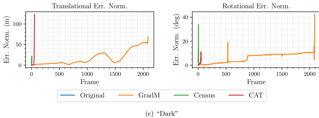
Figure 4.10: Comparison of metric localization errors for the AKITTI/05 sequences. The CAT model was trained using only data from the VKITTI environment.
