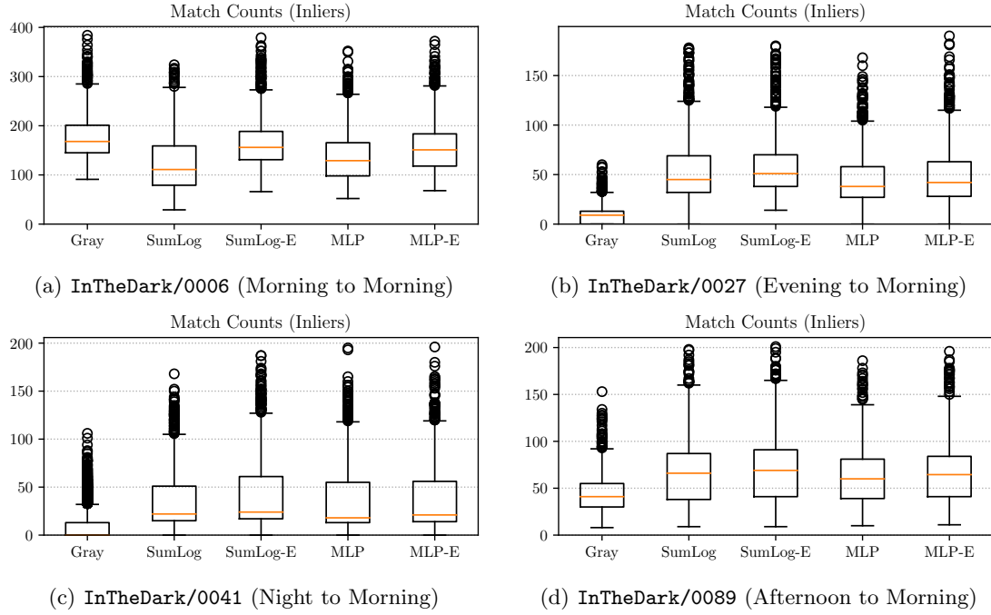
Figure 5.12: Distribution of inlier libviso2 matches for corresponding image pairs from the UTIAS In The Dark dataset, using each RGB-to-grayscale transformation. Orange lines indicate median values.
